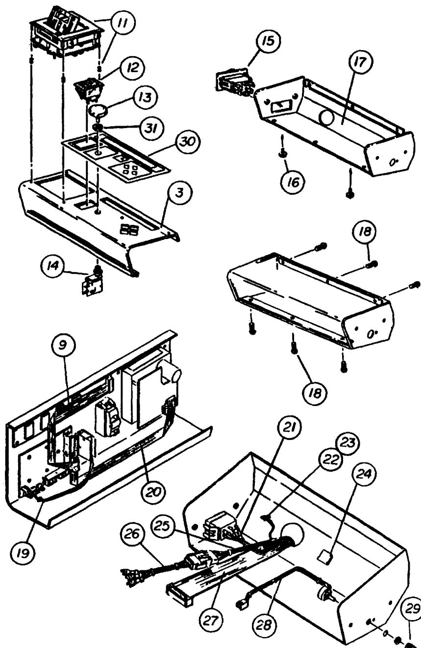
Control Console Assembly 2 - fig. 9
