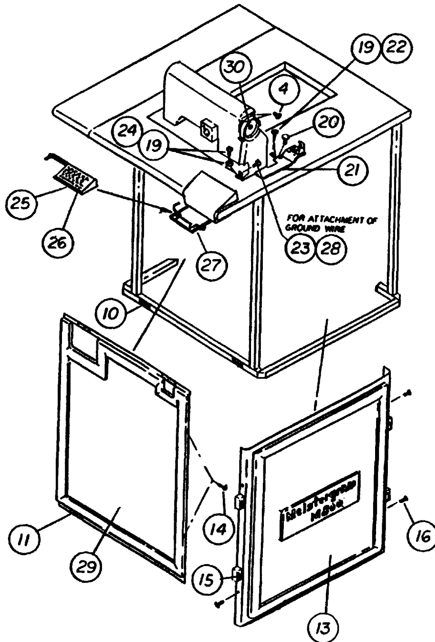
Frame Assembly 2 - fig. 2
